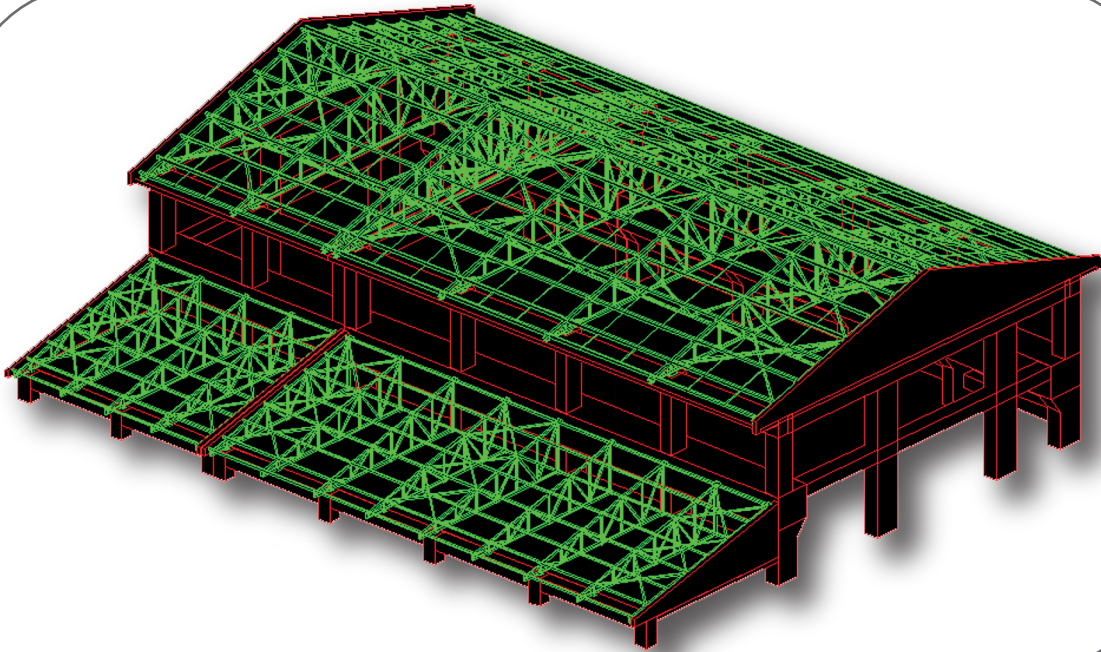
Garzan HEPP Powerhouse Roof
