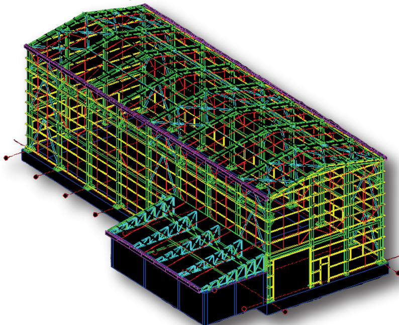
Murat 2 HEPP Powerhouse
