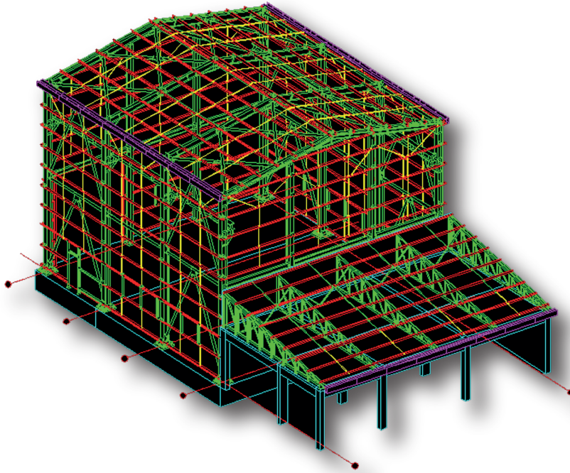
Murat 1 HEPP Powerhouse
